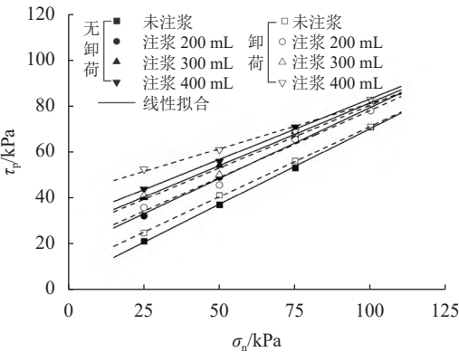
图 3 接触面峰值剪切应力-剪切法向应力拟合曲线 Fig. 3 Fitting curves of interface peak shear stress-applied normal stress
