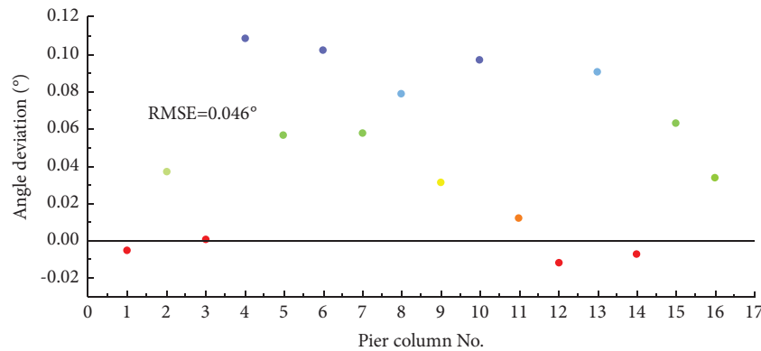
FIGURE 14: Deviation between the perpendicularity of the pier column and the design angle.
